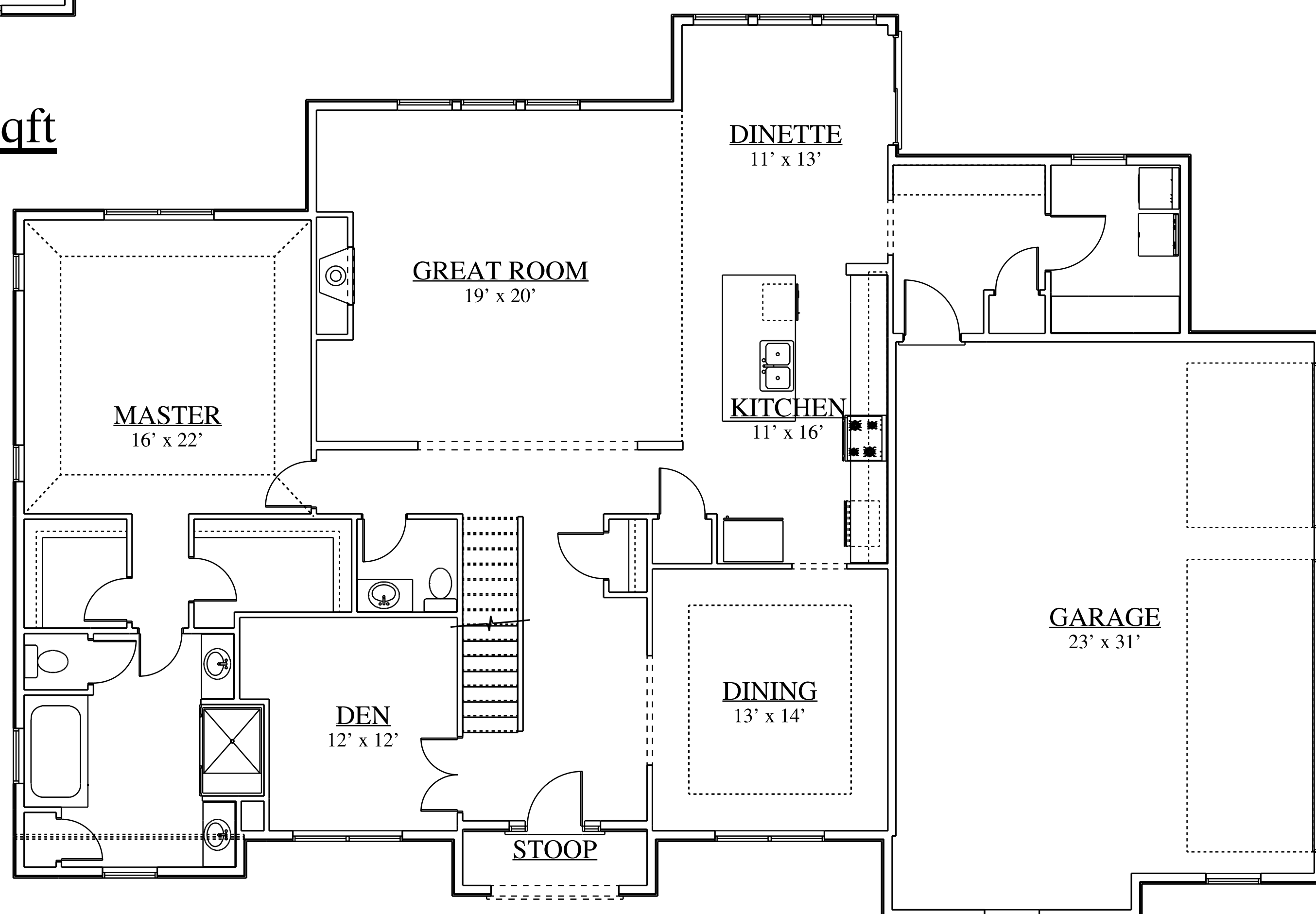
First floor plan 1989 sqft
